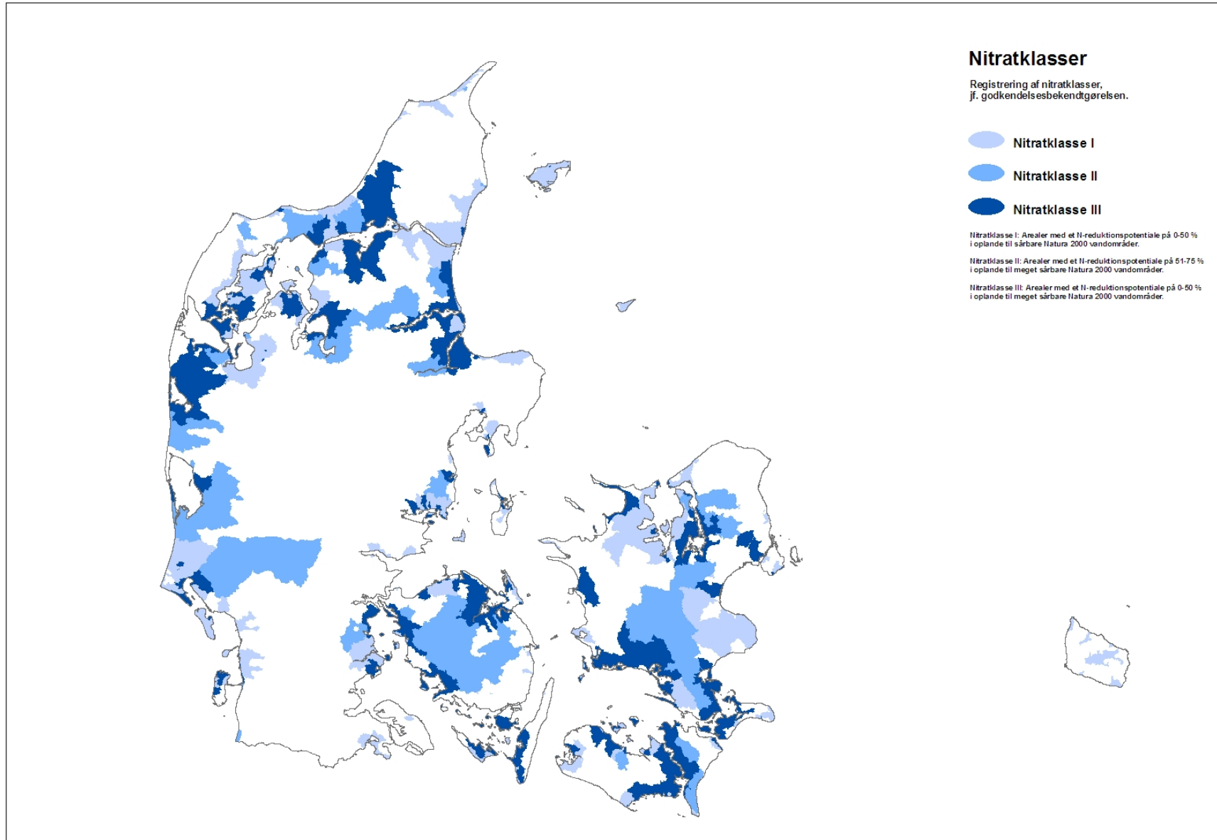
Figure 1. Nitrate class map
